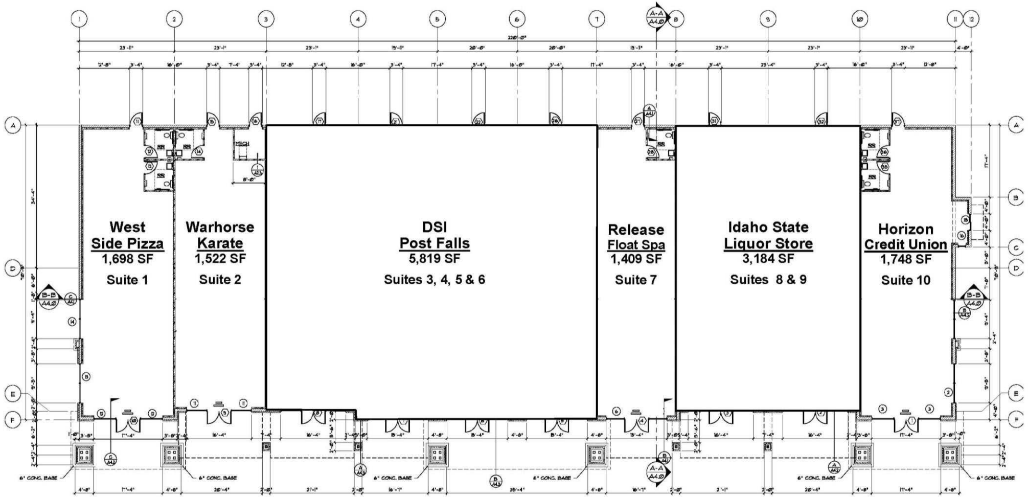
CONSTRUCTION FLOOR PLAN 1/8" = 1'-0"
