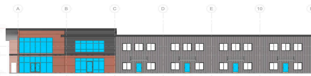
1 North Front Elevation 3/32" = 1'-0"
