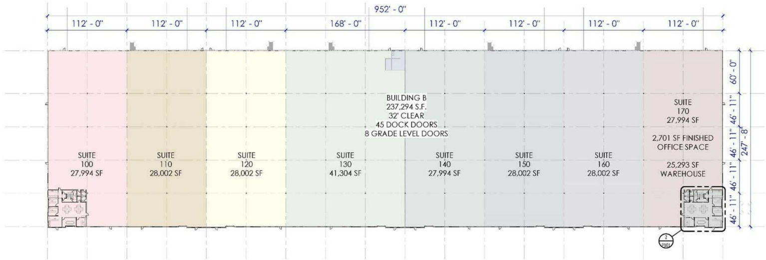
BUILDING B OVERALL AREA PLAN 1" = 40'-0"
