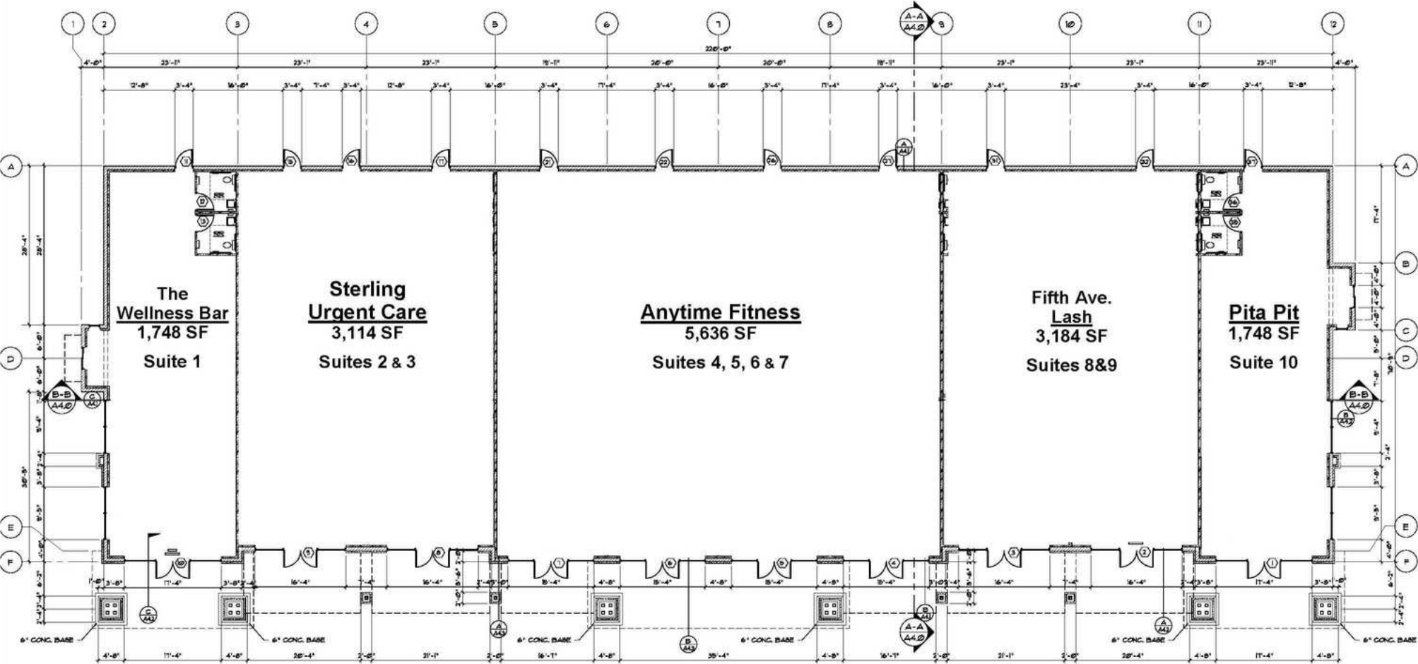
CONSTRUCTION FLOOR PLAN 1/8" = 1'-0"
