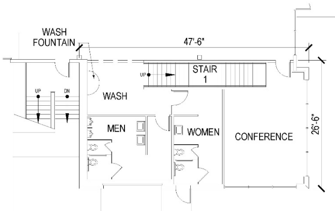
South Office Area – 1 st Floor
