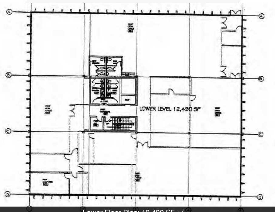
Lower Floor Plan: 12,490 SF +/-
