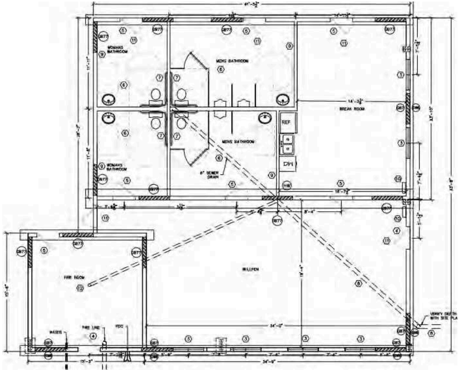
INTERIOR FRAMING PLAN
