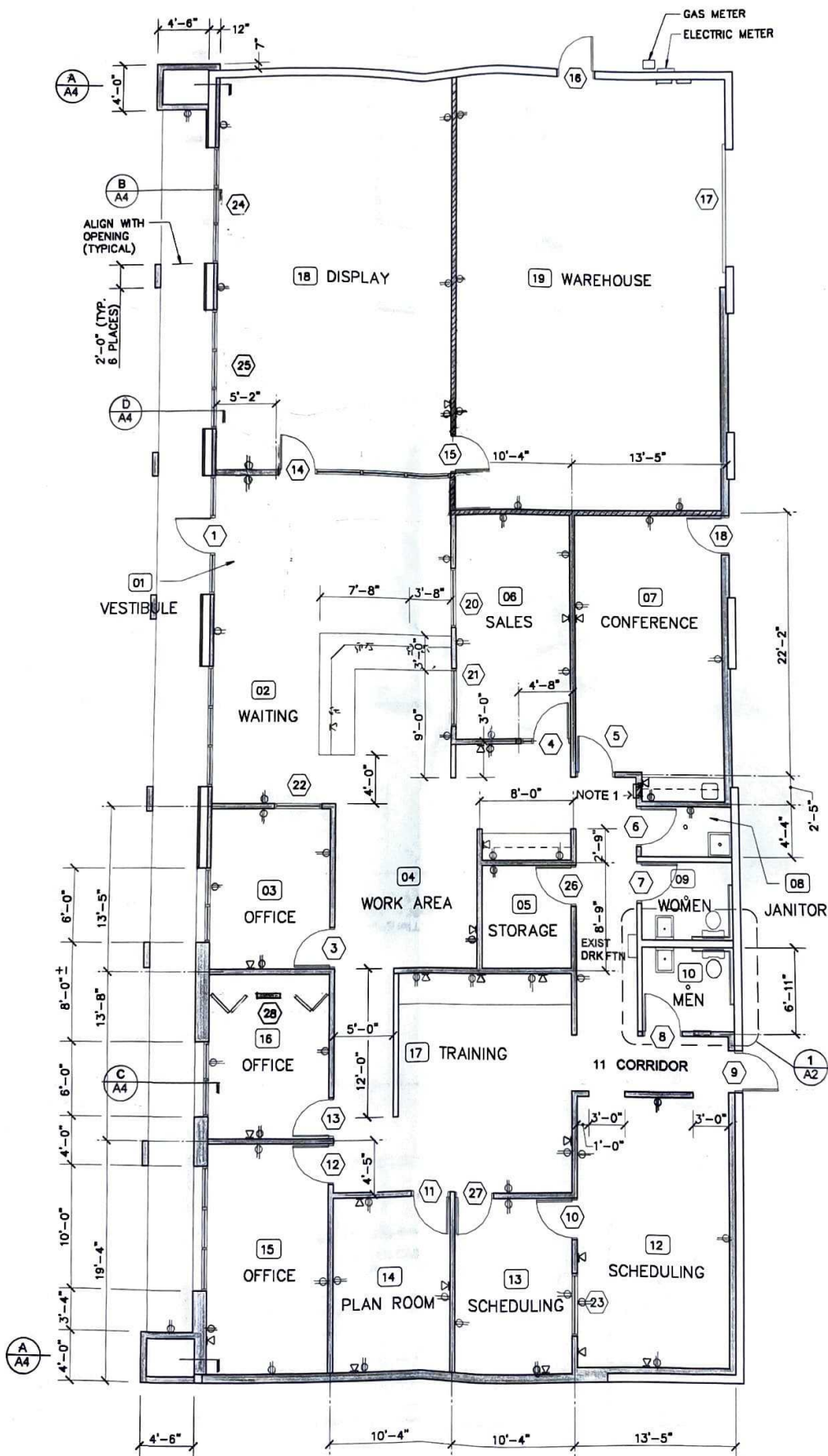
Floor Plan
