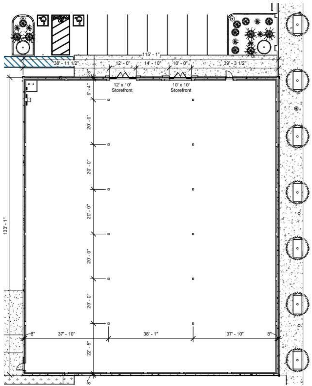
1 Building Layout 1/16" = 1'-0"
