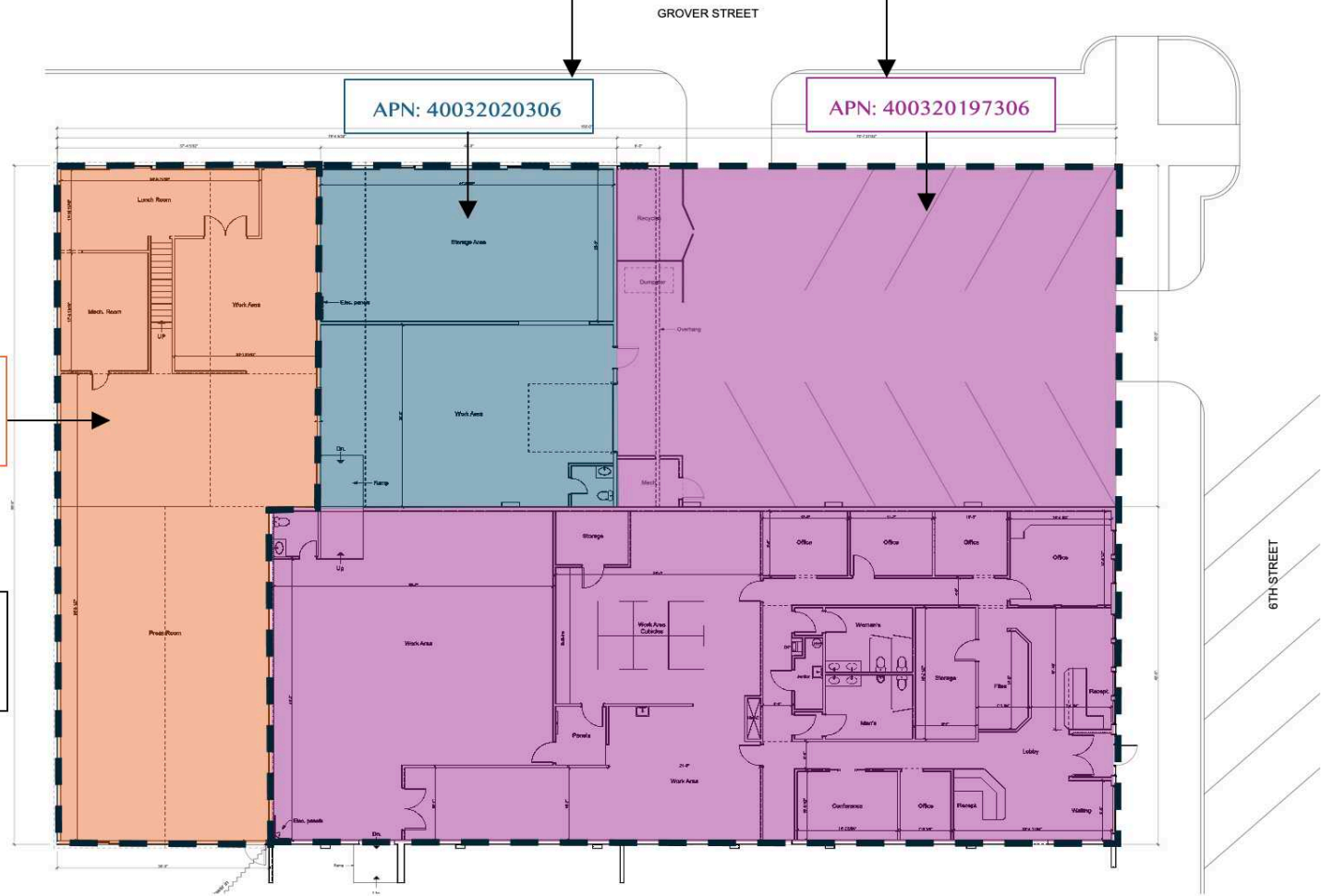
GROUND FLOOR PLAN - Existing 1/8" = 1' - 0"
