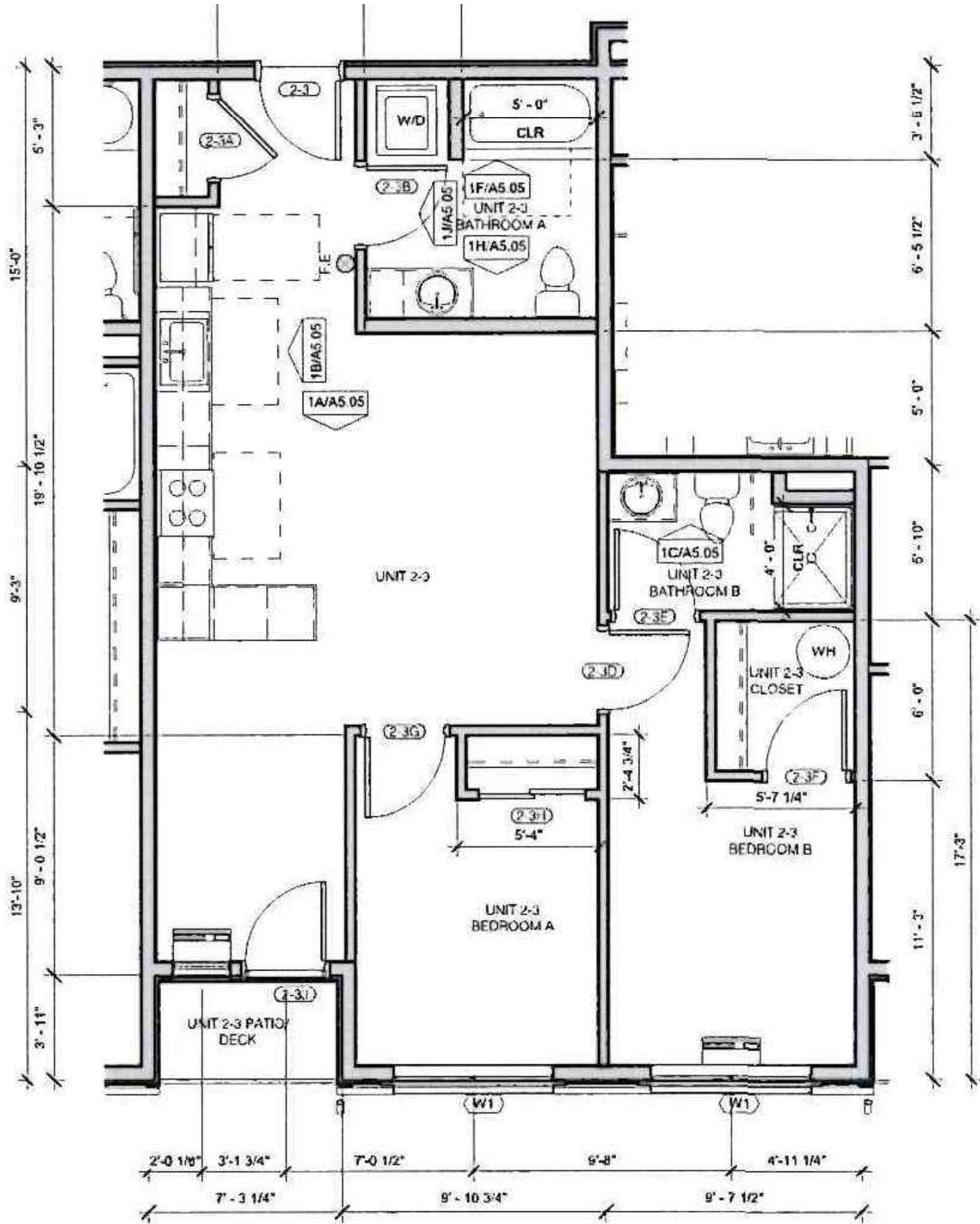
1 UNIT 2-3 ENLARGED PLAN SCALE: 1/4" = 1'-0"
