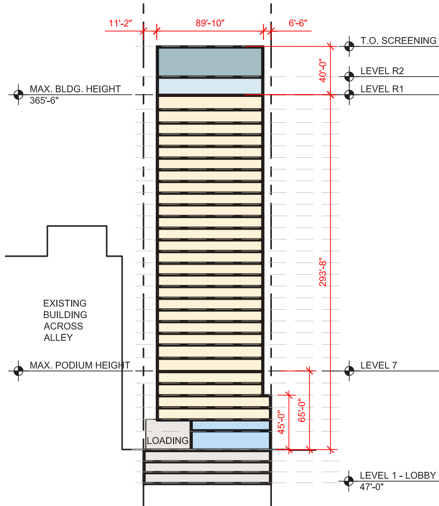
OPTION 1: NORTH FACING BUILDING SECTION
